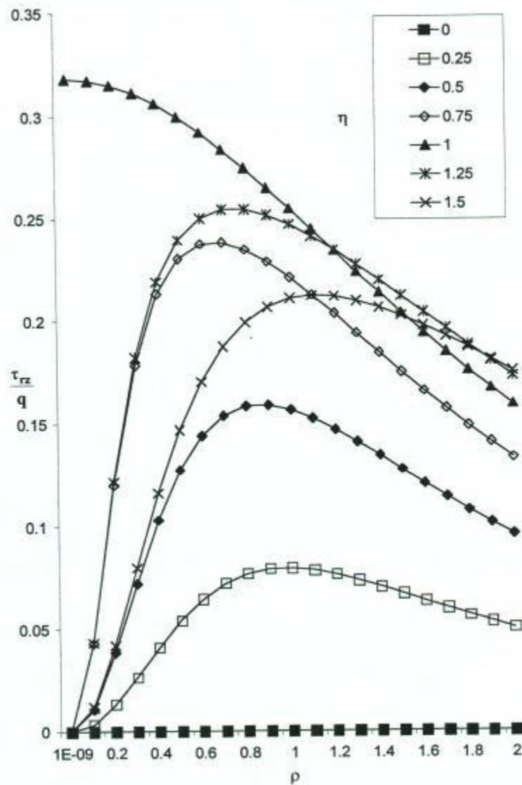
Figure 5: The value of \tau_{rz} as calculated from equation 2.
