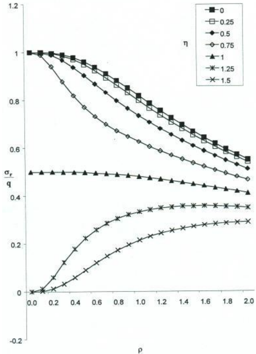
Figure 4: The value of \sigma_r/q as calculated with equation 1.
